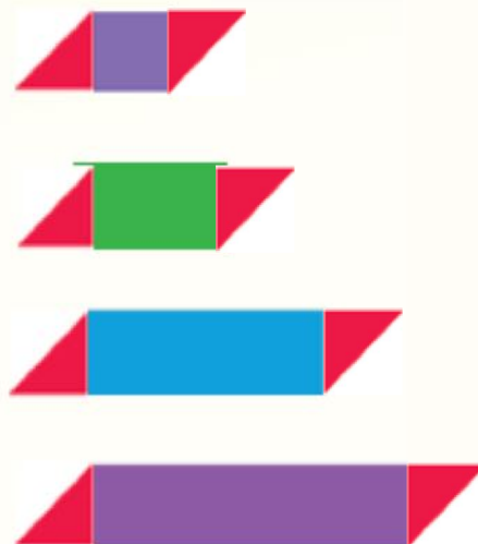
parallelograms
