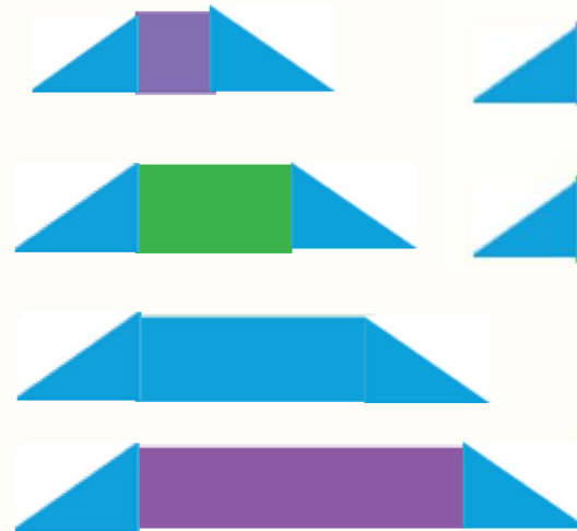
trapezoids
